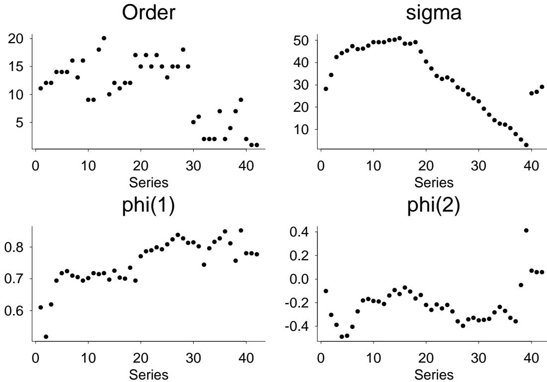
Fig. 6.8. Statistics for a sequence of subseries.
