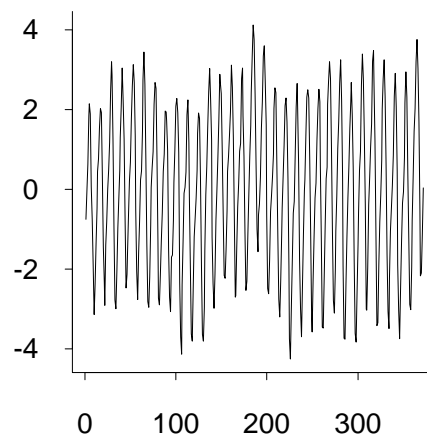
Cubic trend removed
