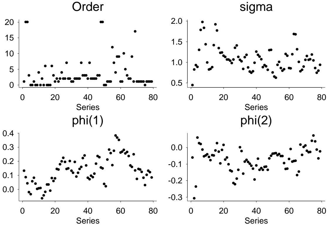
Fig. 6.21. AR models fitted to 79 subseries of the S&P data.
