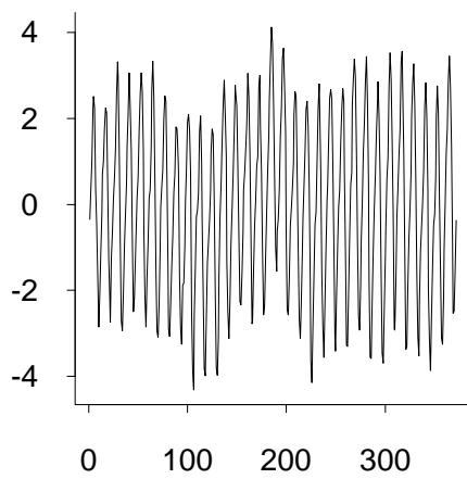
Quadratic trend removed
