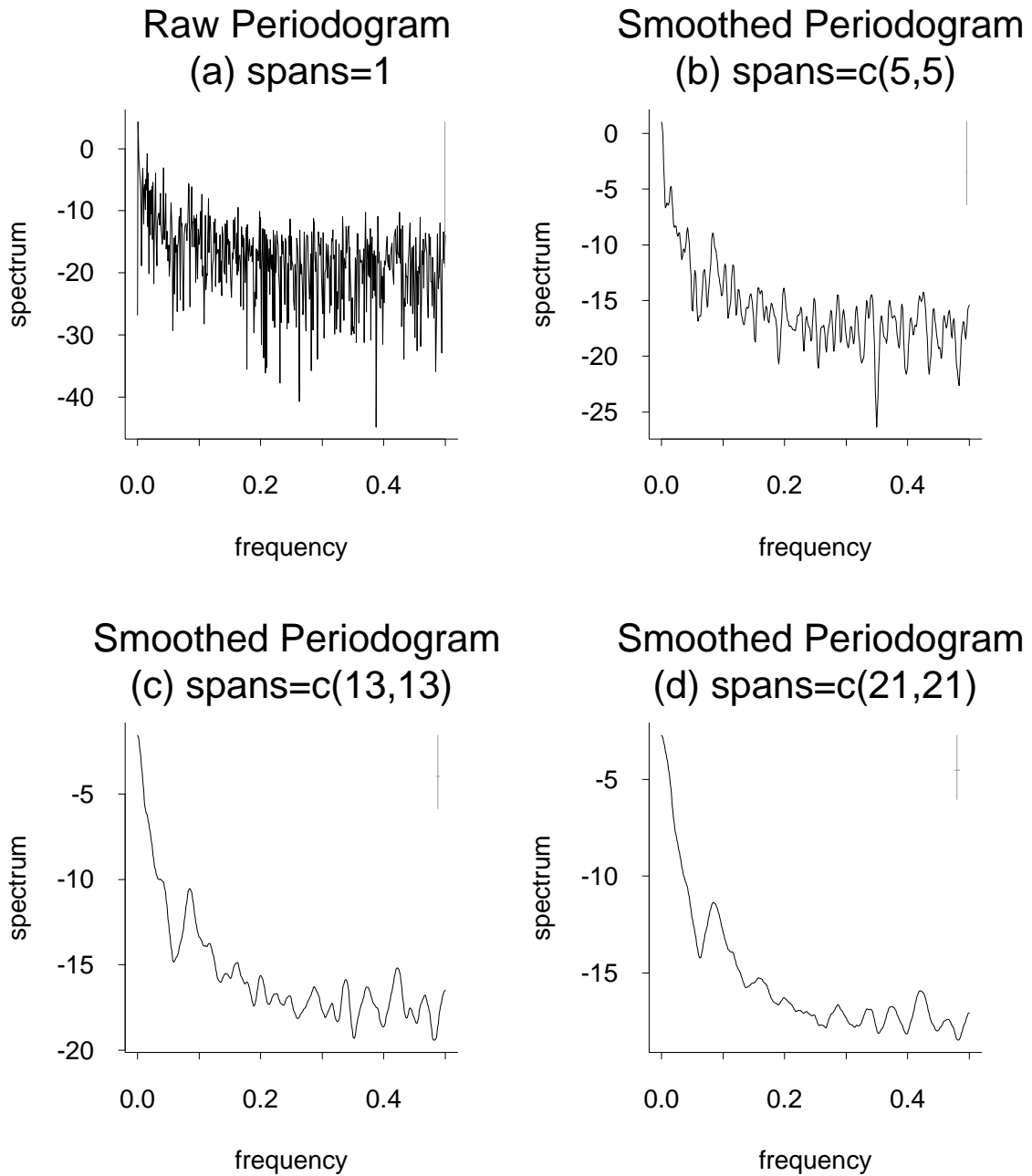
Fig. 5.7: Temperature Spectra
