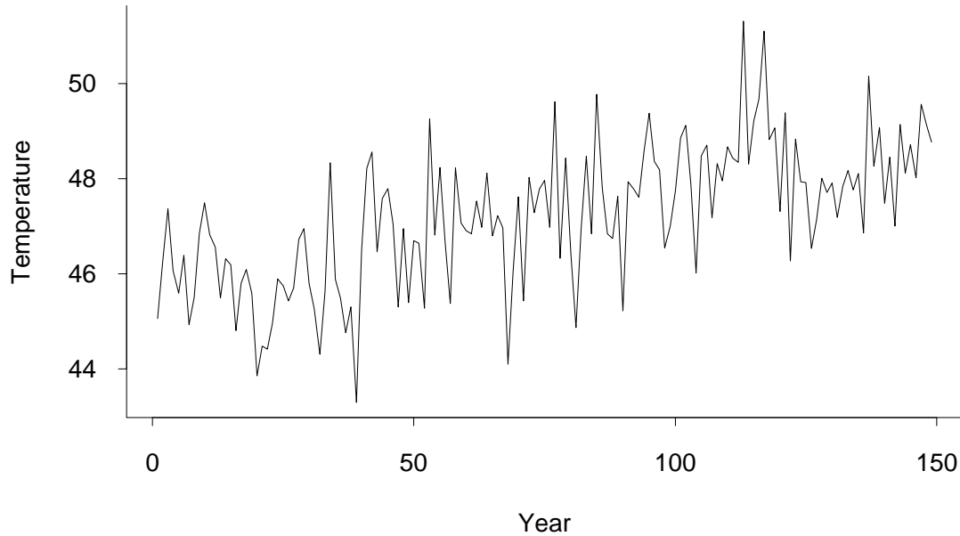
Fig. 6.9. Annual mean temperature in Amherst, MA.
