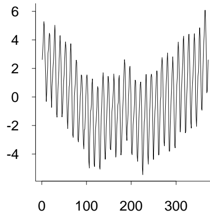
Linear trend removed
